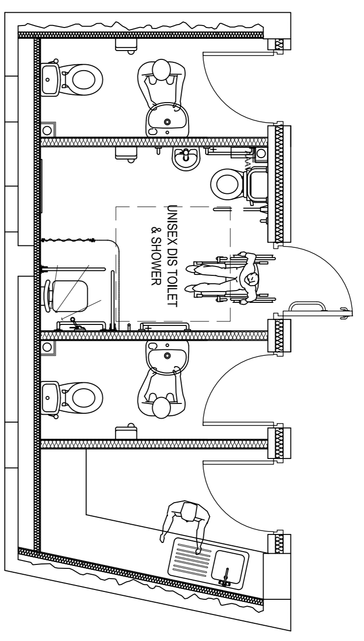
Refurbished Toilet Layout Scale 1:50
