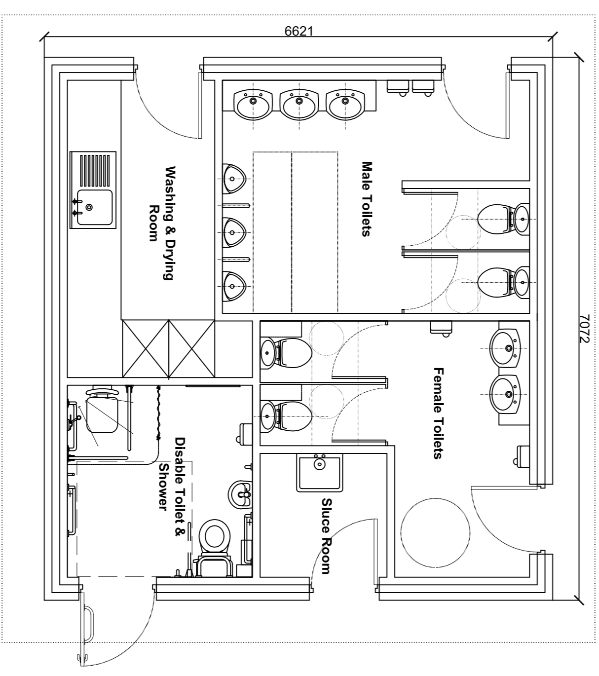
Proposed New Toilet Facility Layout Scale 1:50
