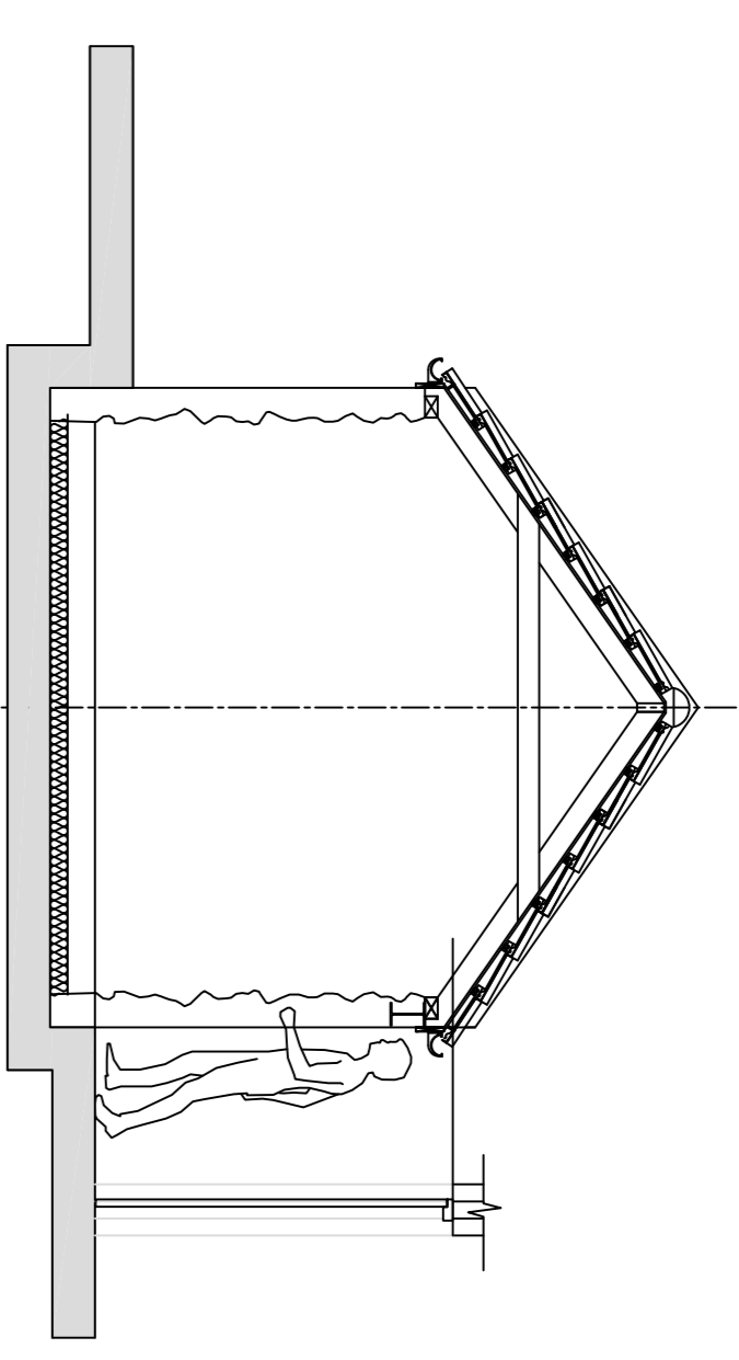
Sketch Section Layout Scale 1:50
