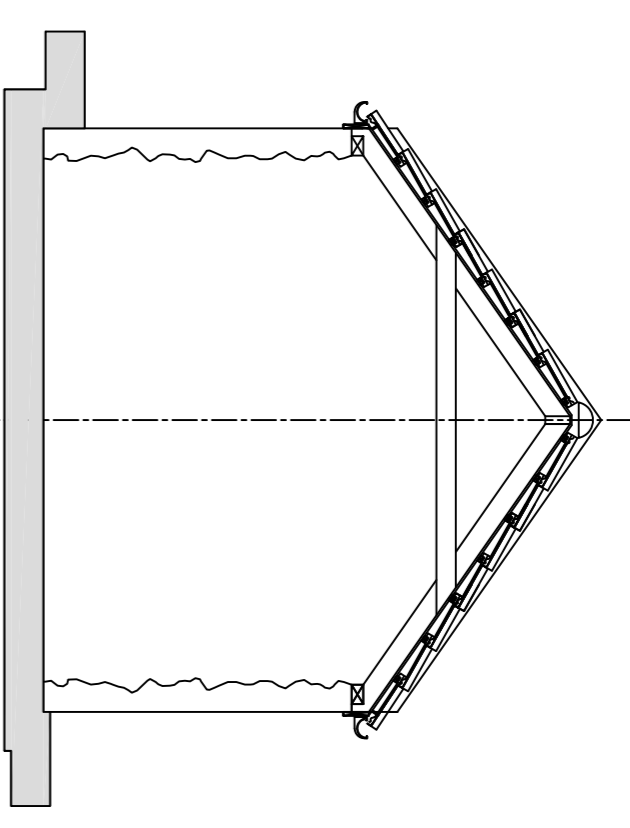
Existing Building Section Scale 1:50
